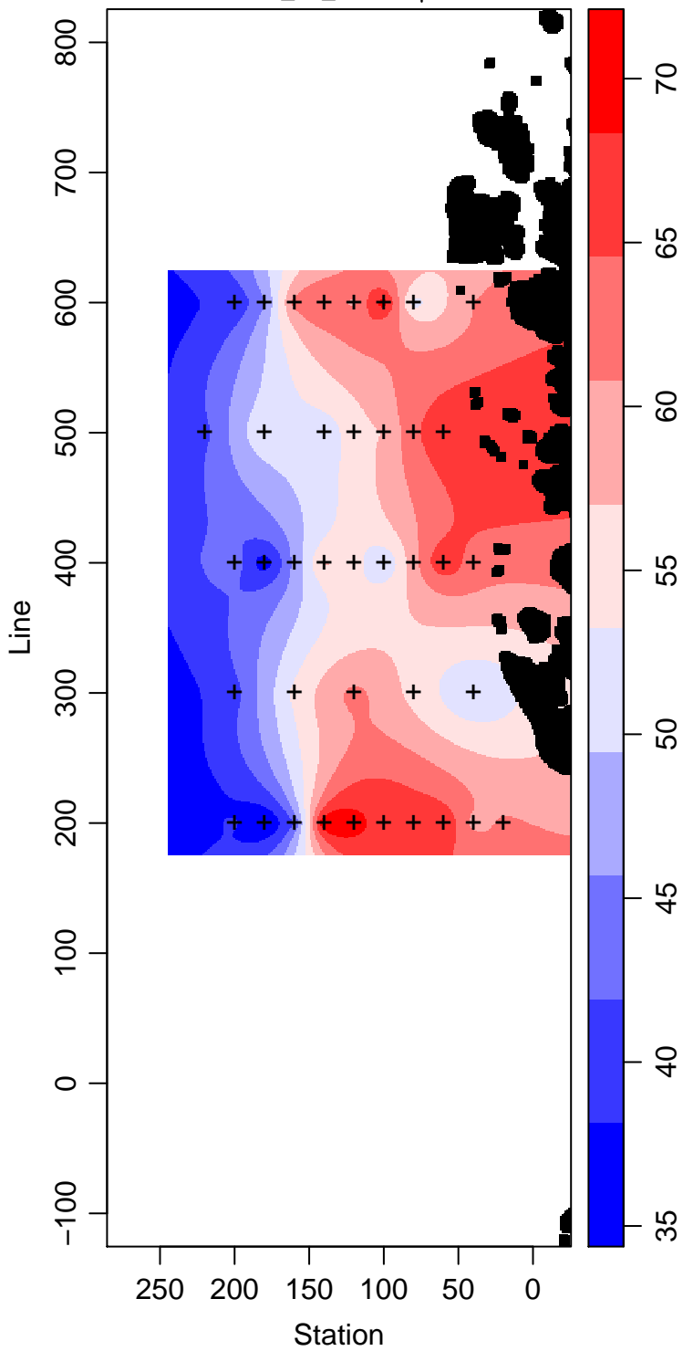
LMG01-01_40_Silicate \mu\text{ mol L}^{-1}
