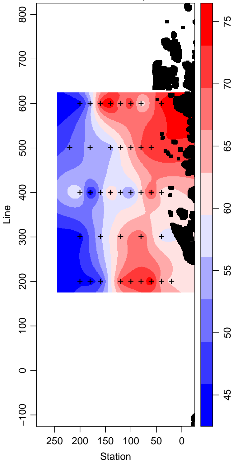
LMG01-01_55_Silicate \mu\text{ mol L}^{-1}
