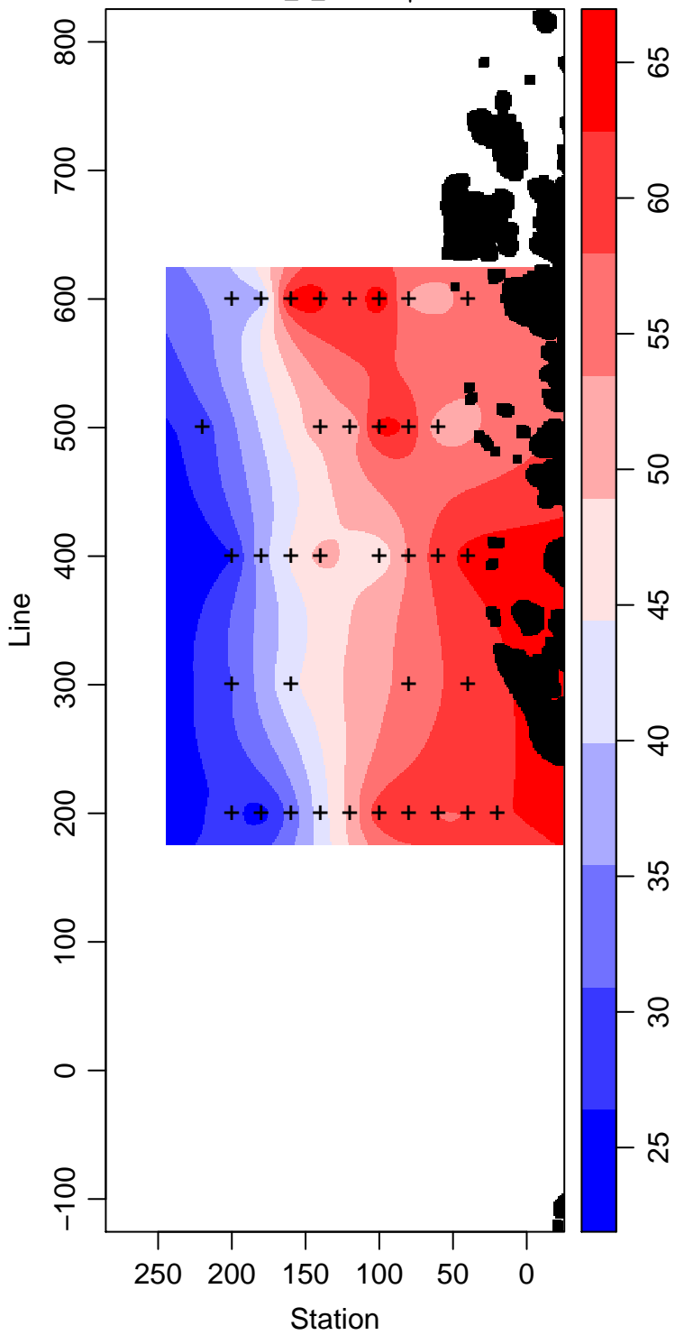
LMG01-01_5_Silicate \mu\text{ mol L}^{-1}
