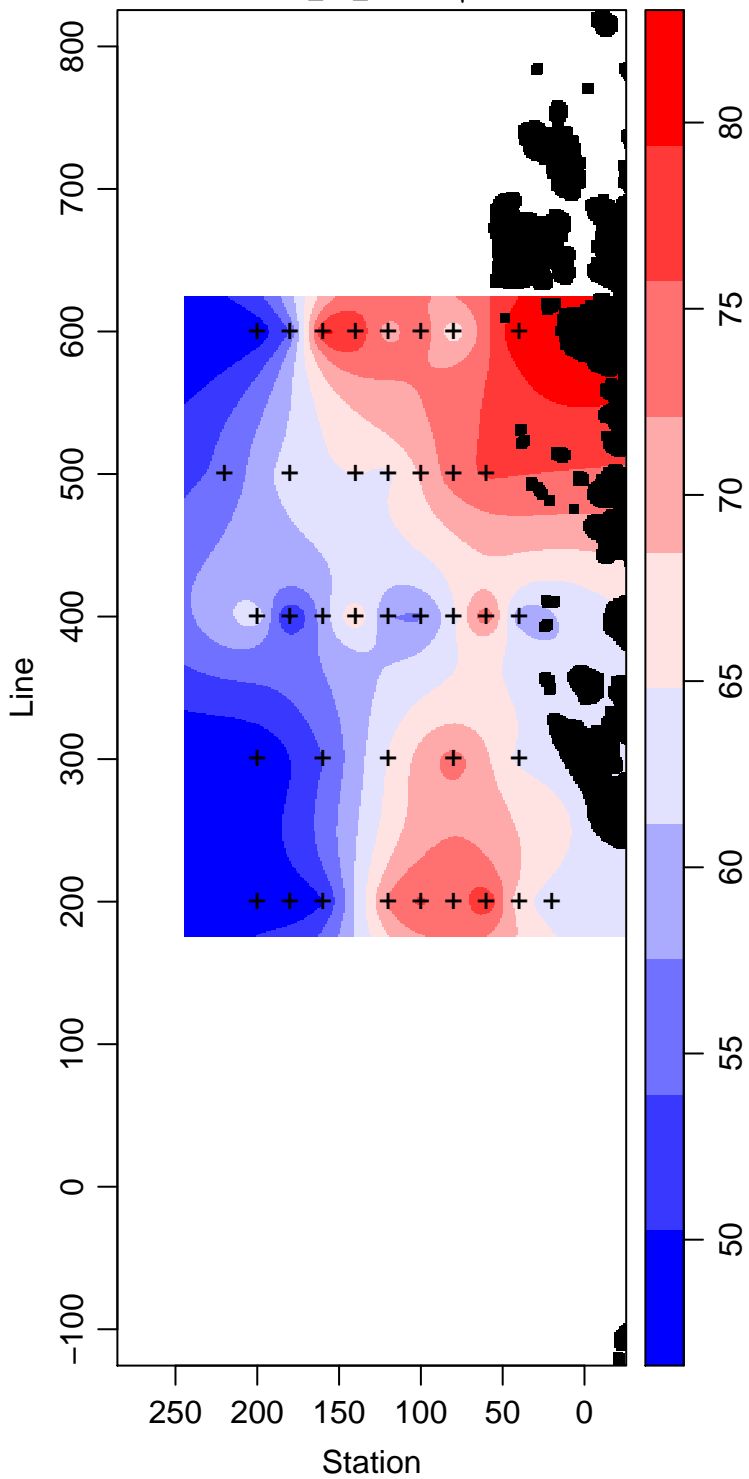
LMG01-01_65_Silicate \mu\text{ mol L}^{-1}
