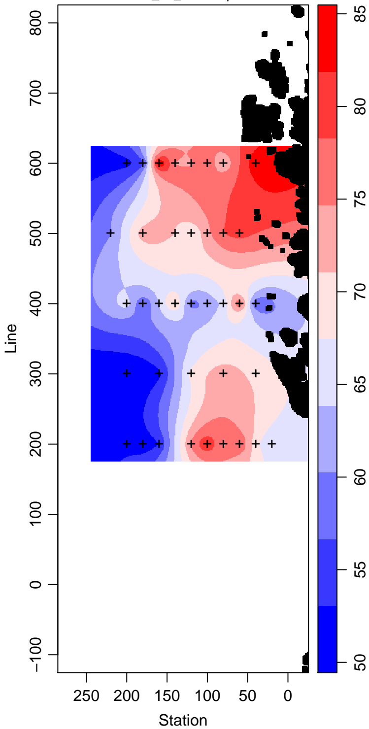
LMG01-01_75_Silicate \mu\text{ mol L}^{-1}
