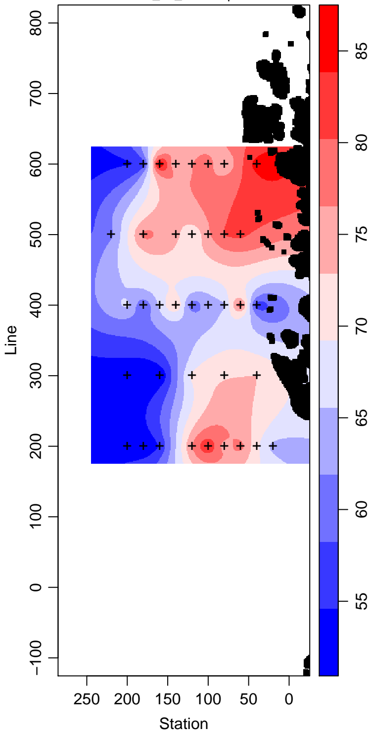
LMG01-01_80_Silicate \mu\text{ mol L}^{-1}
