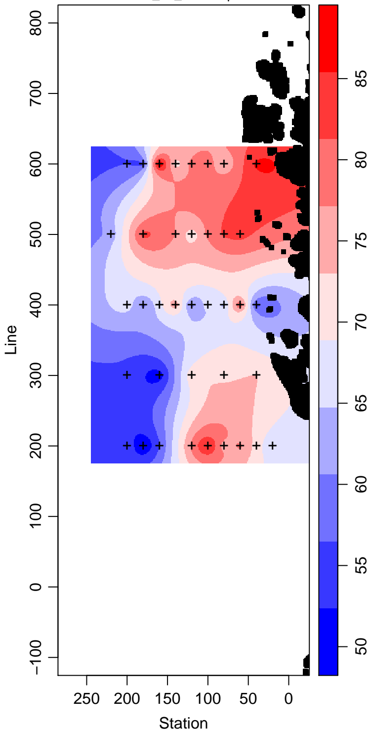
LMG01-01_85_Silicate \mu\text{ mol L}^{-1}
