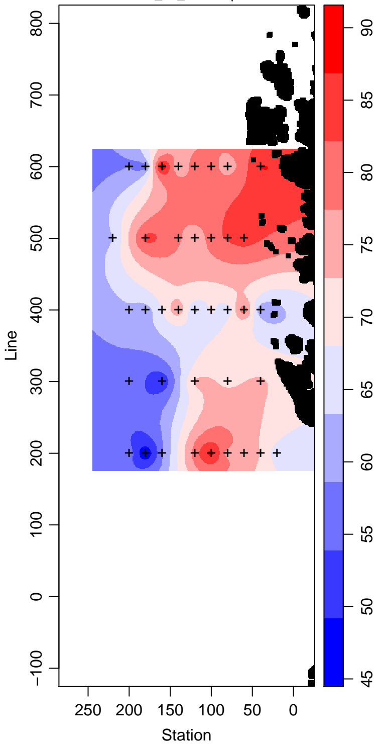
LMG01-01_90_Silicate \mu\text{ mol L}^{-1}
