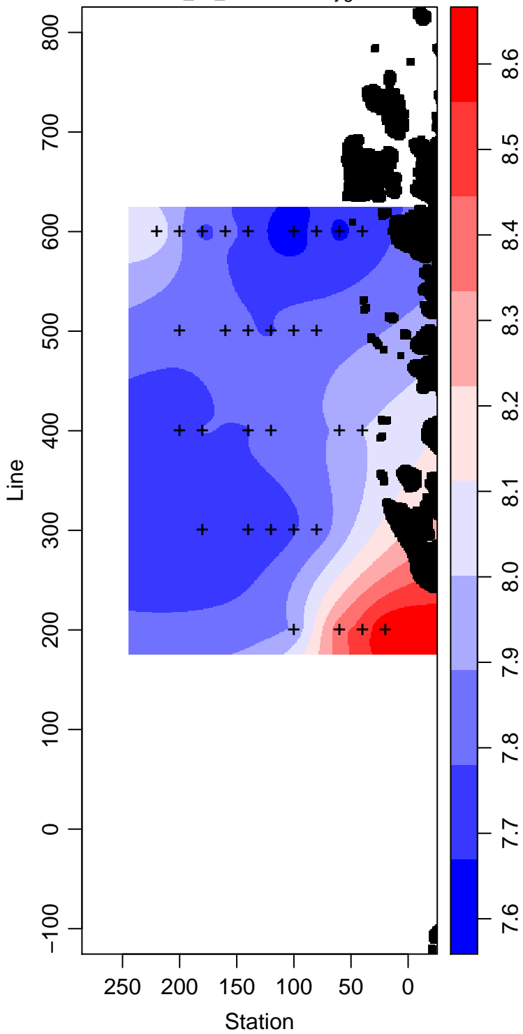
LMG02-01_35_Dissolved.Oxygen ml L -1
