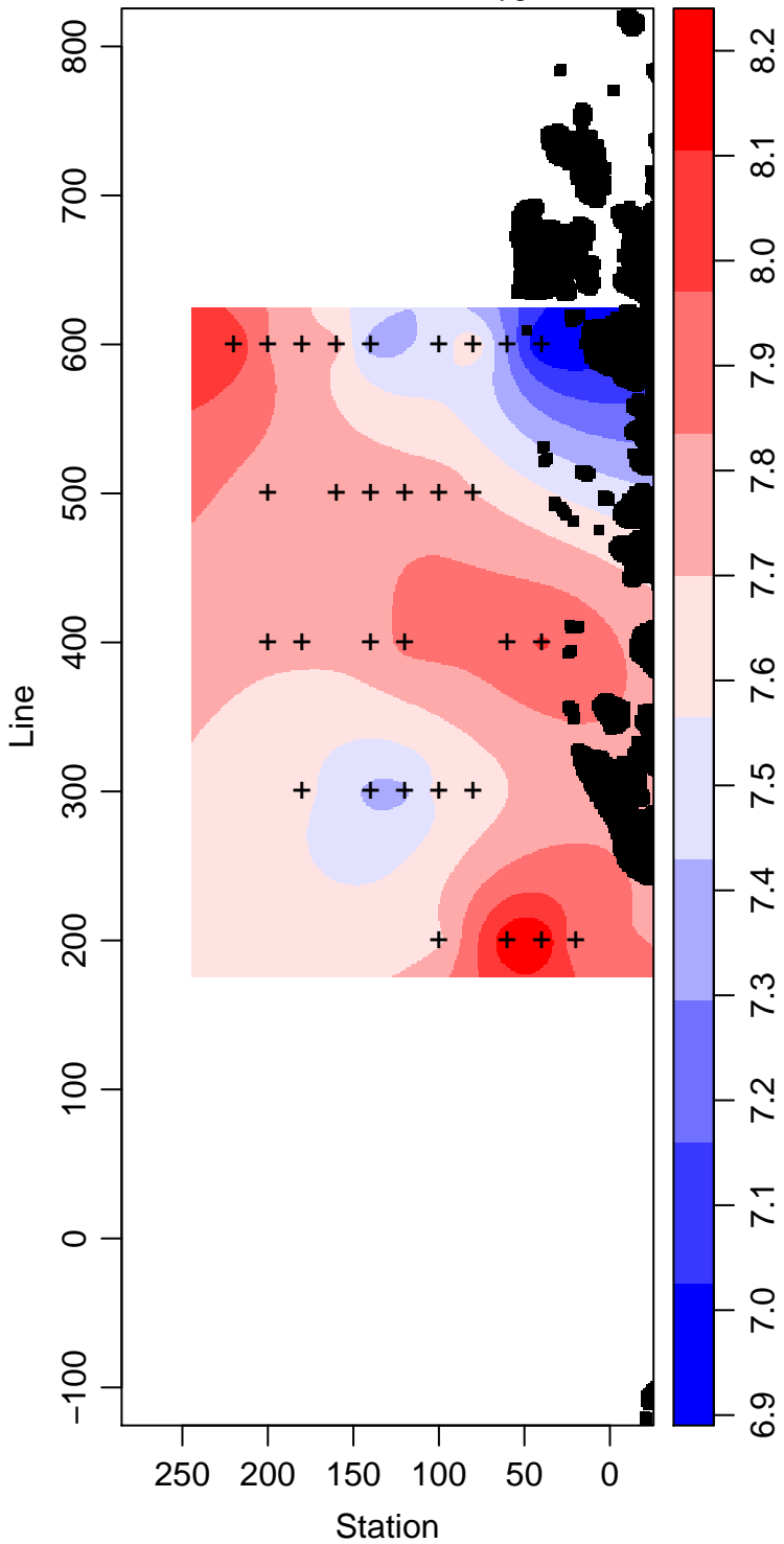
LMG02-01_45_Dissolved.Oxygen ml L -1
