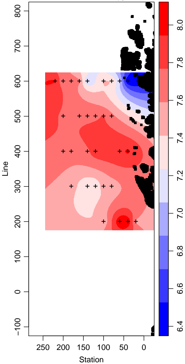
LMG02-01_50_Dissolved.Oxygen ml L -1
