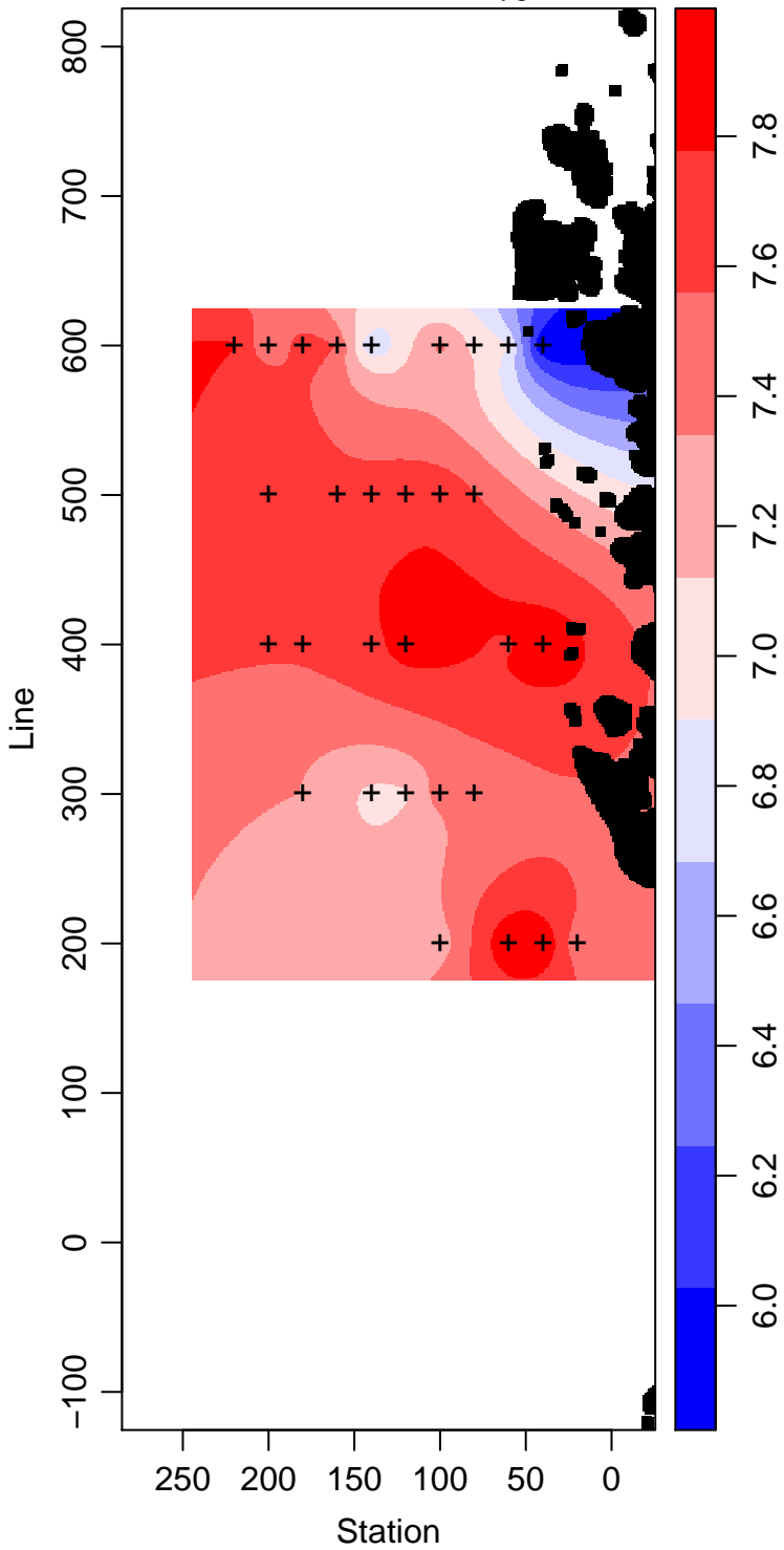
LMG02-01_55_Dissolved.Oxygen ml L -1
