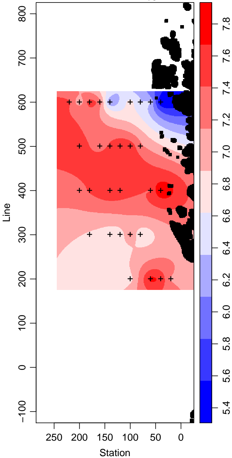
LMG02-01_65_Dissolved.Oxygen ml L -1
