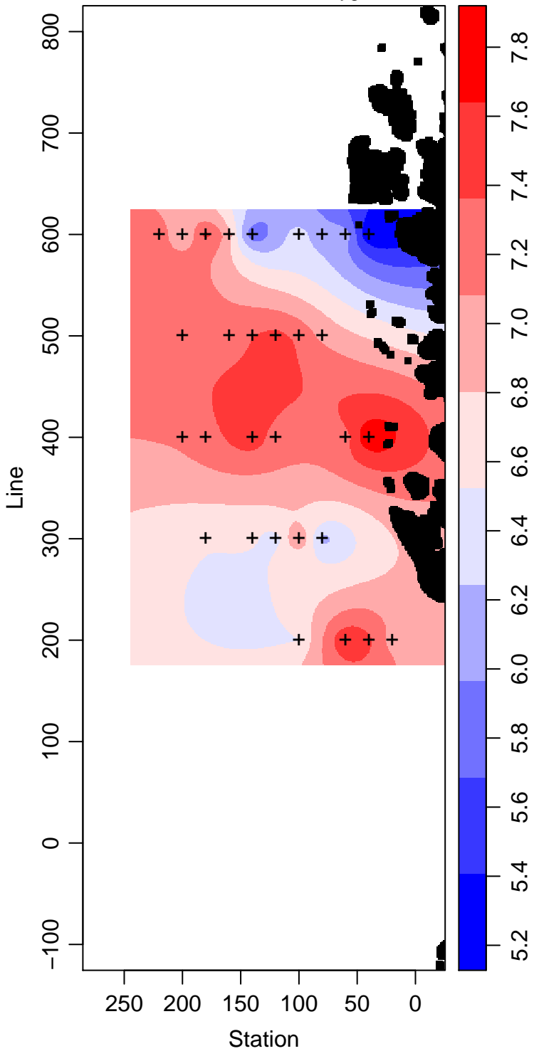
LMG02-01_70_Dissolved.Oxygen ml L -1
