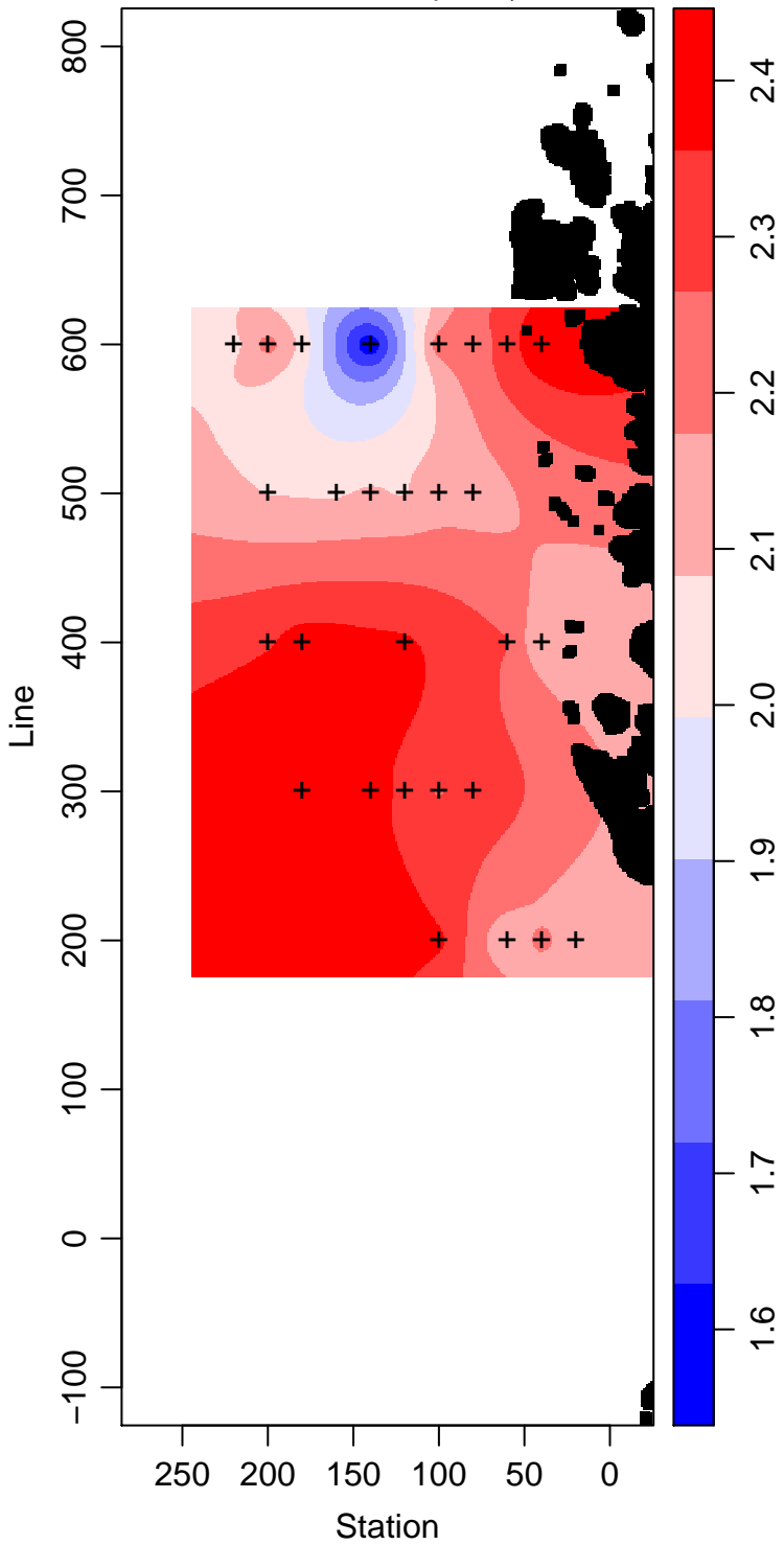
LMG02-01_100_Phosphate \mu\text{ mol L}^{-1}
