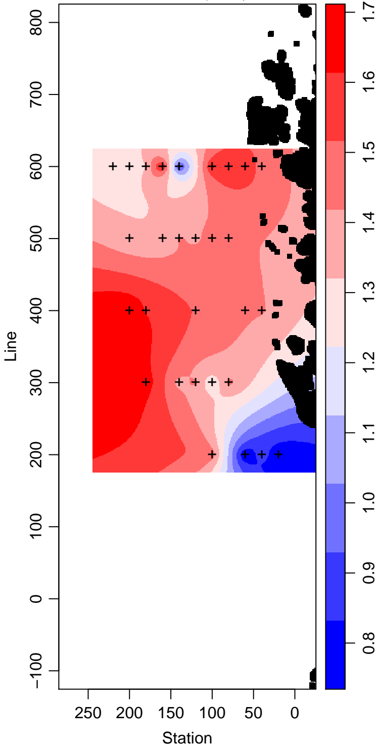
LMG02-01_15_Phosphate \mu\text{ mol L}^{-1}
