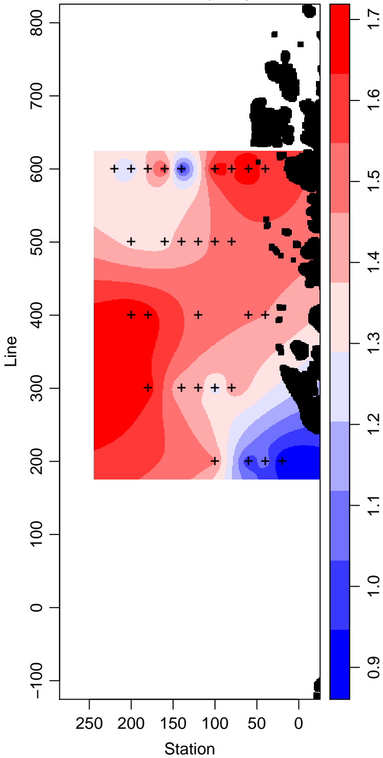
LMG02-01_25_Phosphate \mu\text{ mol L}^{-1}
