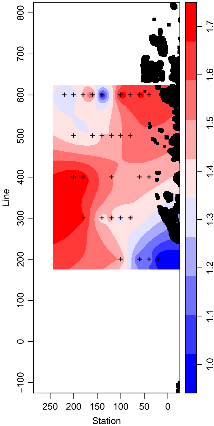
LMG02-01_30_Phosphate \mu\text{ mol L}^{-1}
