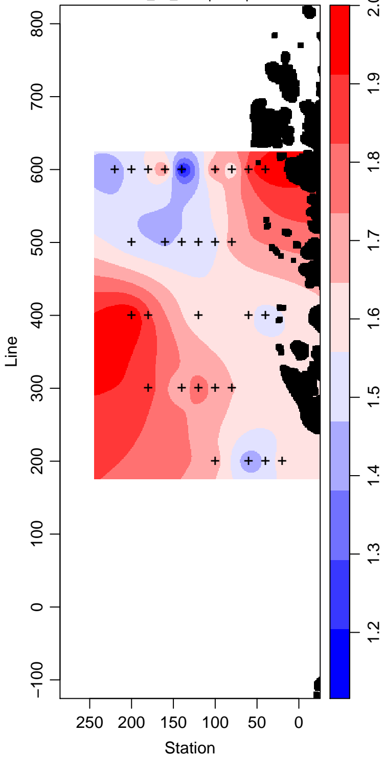
LMG02-01_45_Phosphate \mu\text{ mol L}^{-1}
