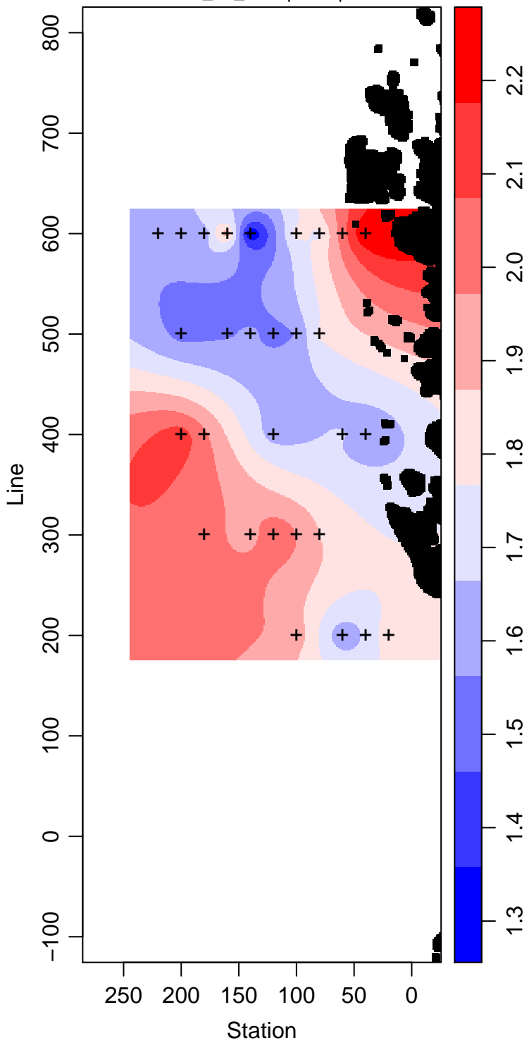
LMG02-01_55_Phosphate \mu\text{ mol L}^{-1}
