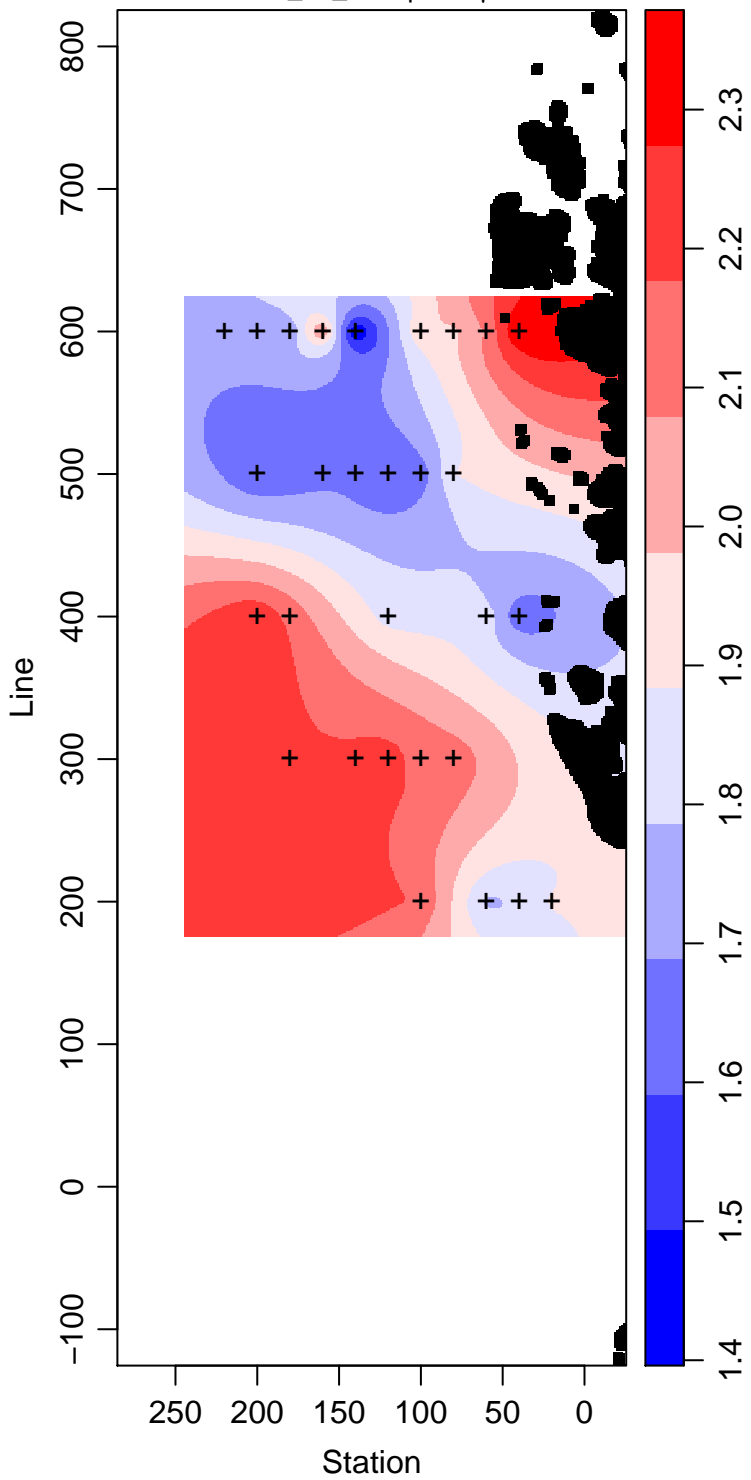
LMG02-01_65_Phosphate \mu\text{ mol L}^{-1}
