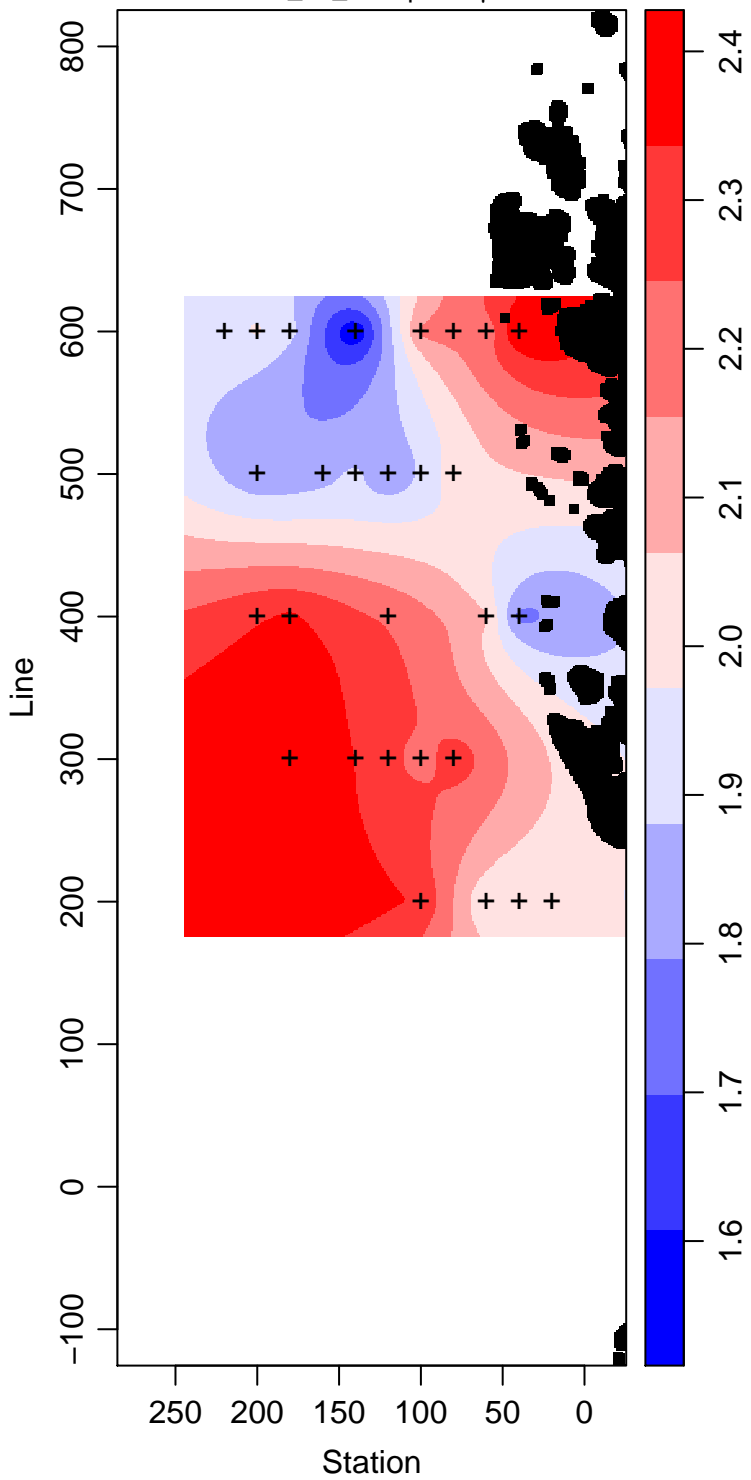
LMG02-01_80_Phosphate \mu\text{ mol L}^{-1}
