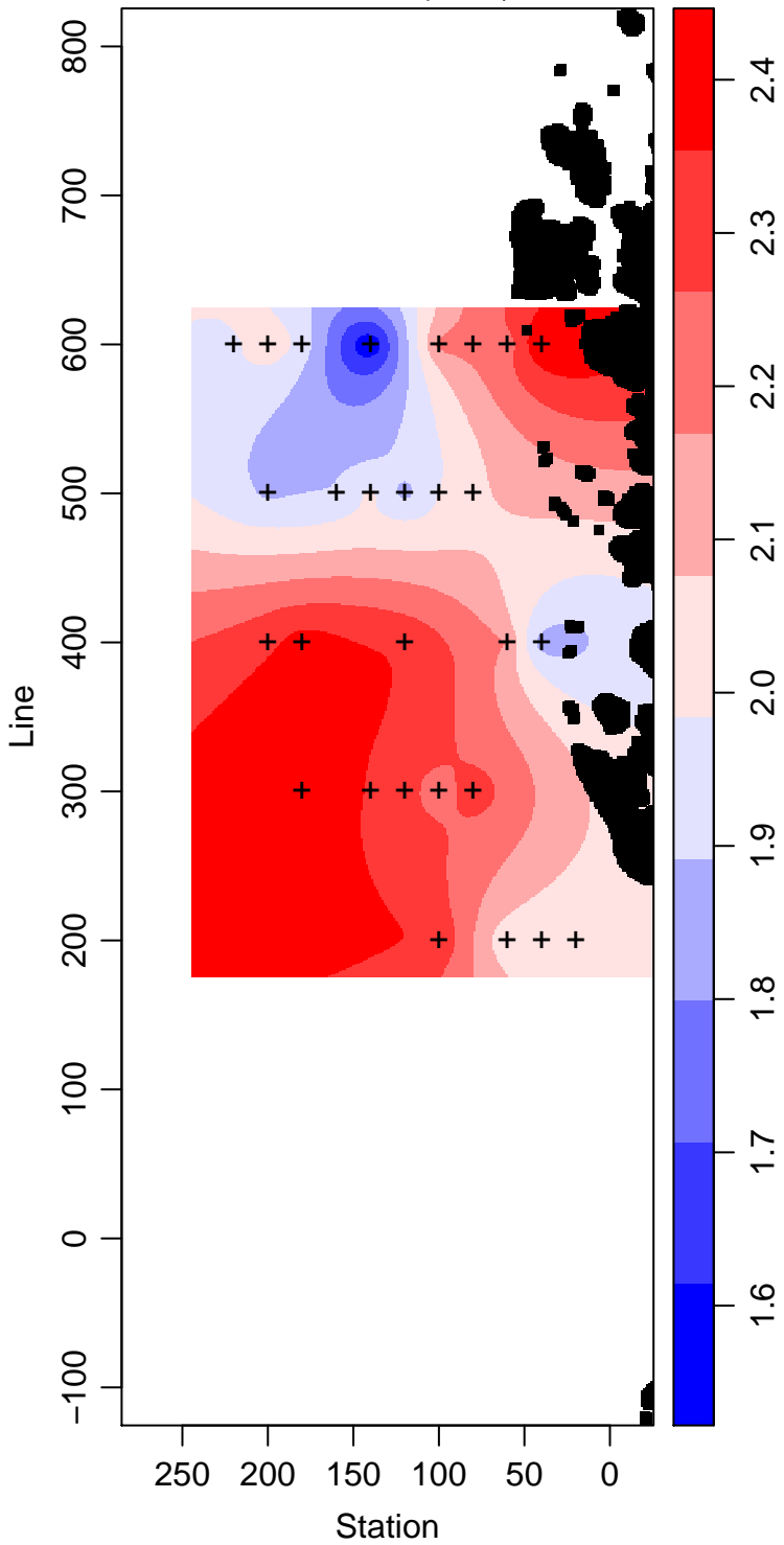
LMG02-01_85_Phosphate \mu\text{ mol L}^{-1}
