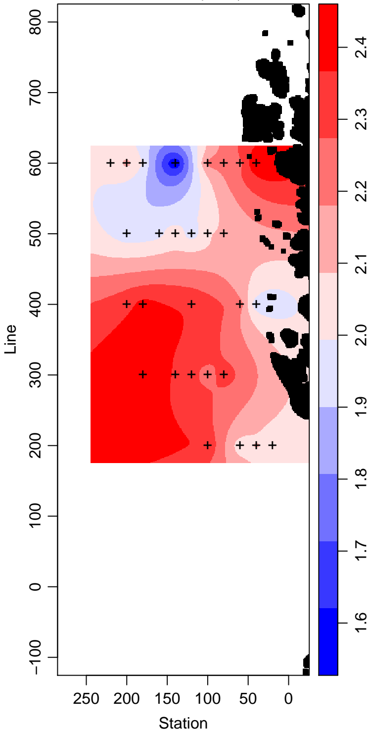
LMG02-01_90_Phosphate \mu\text{ mol L}^{-1}
