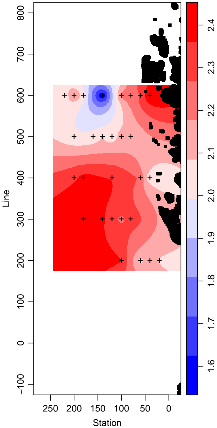
LMG02-01_95_Phosphate \mu\text{ mol L}^{-1}
