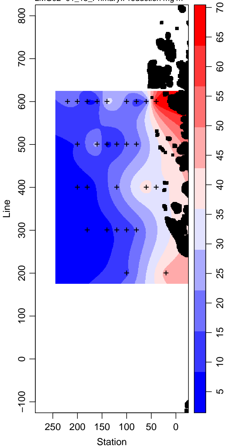
LMG02-01_15_Primary.Production mg m -3
