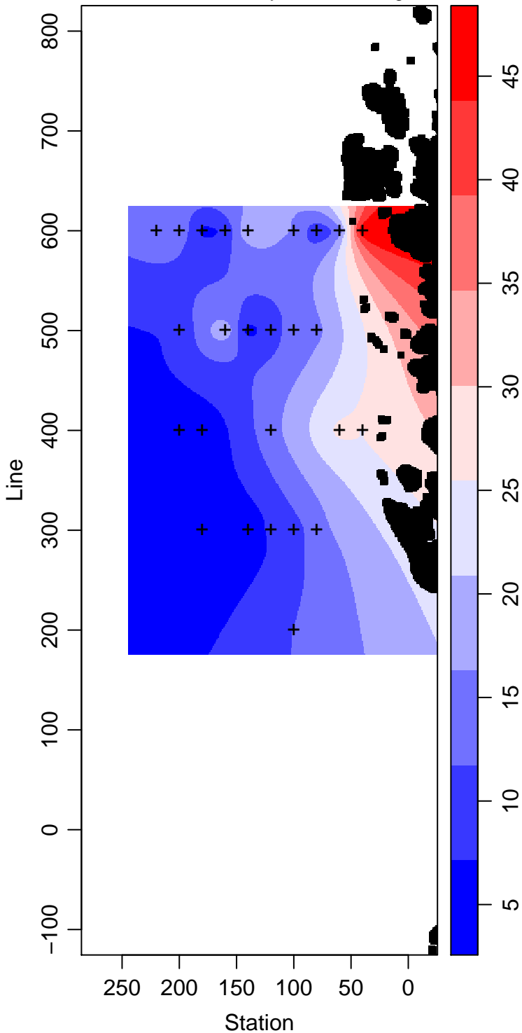
LMG02-01_20_Primary.Production mg m -3
