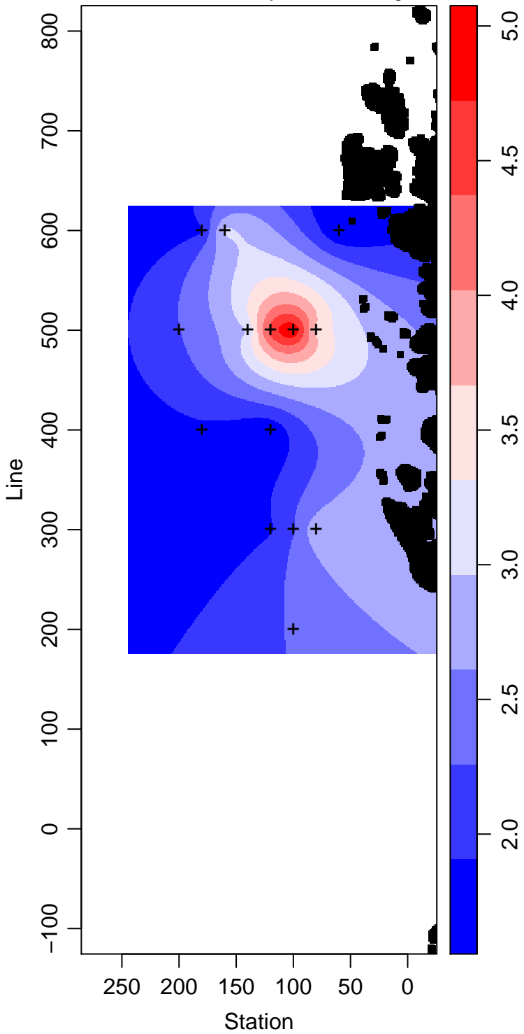
LMG02-01_50_Primary.Production mg m -3
