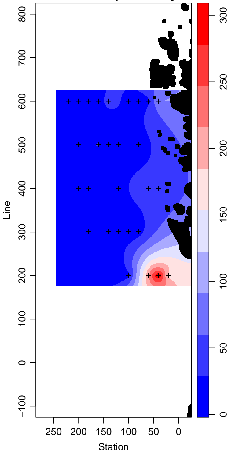
LMG02-01_5_Primary.Production mg m -3
