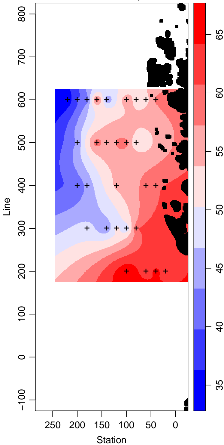
LMG02-01_15_Silicate \mu\text{ mol L}^{-1}
