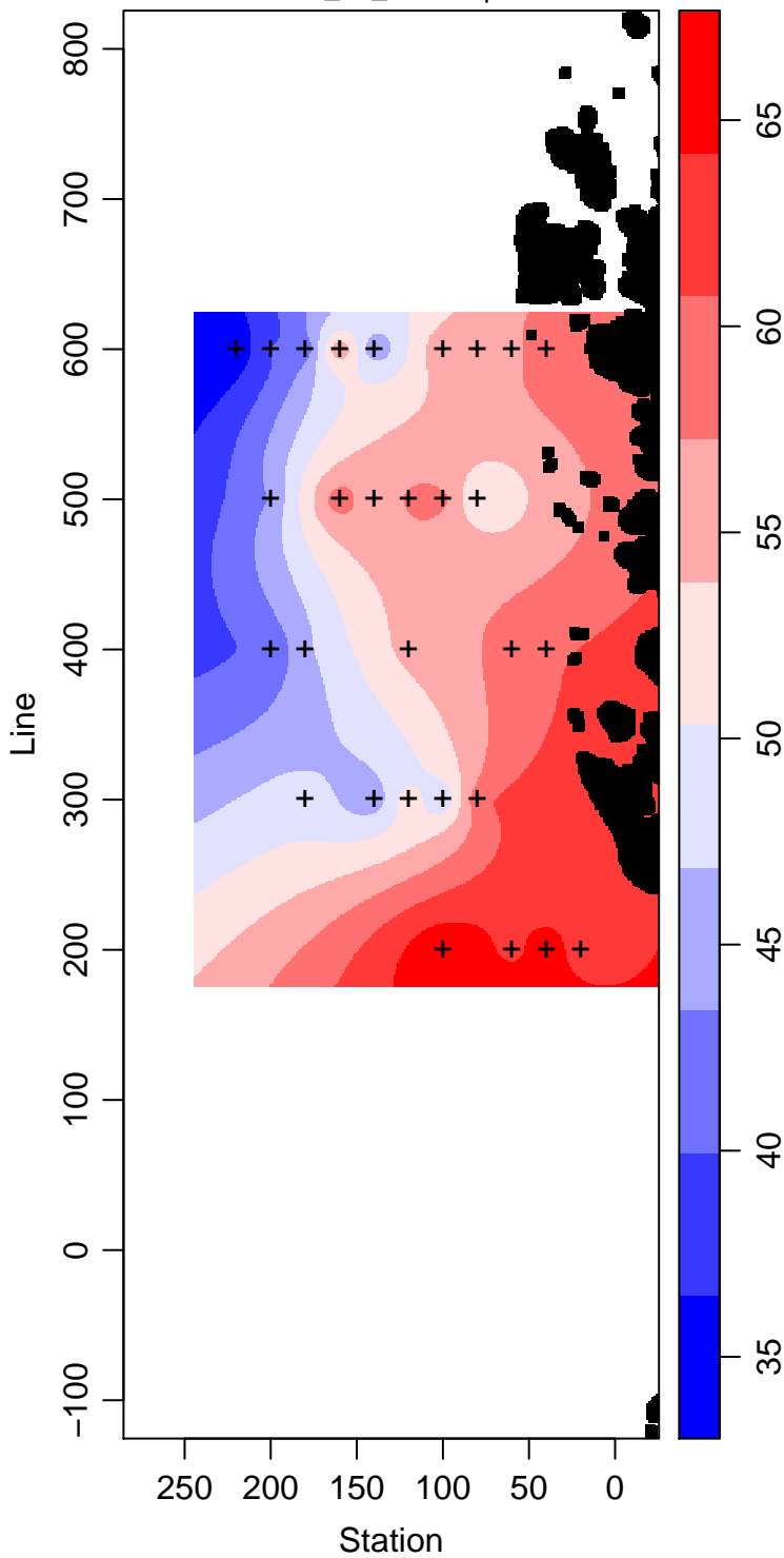
LMG02-01_20_Silicate \mu\text{ mol L}^{-1}
