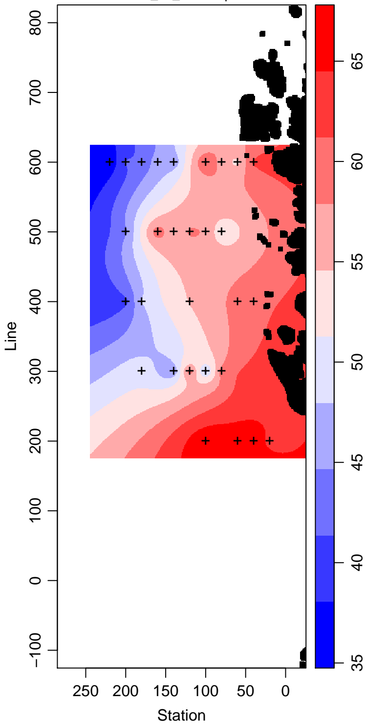
LMG02-01_30_Silicate \mu\text{ mol L}^{-1}
