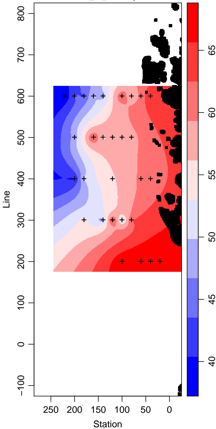
LMG02-01_40_Silicate \mu\text{ mol L}^{-1}
