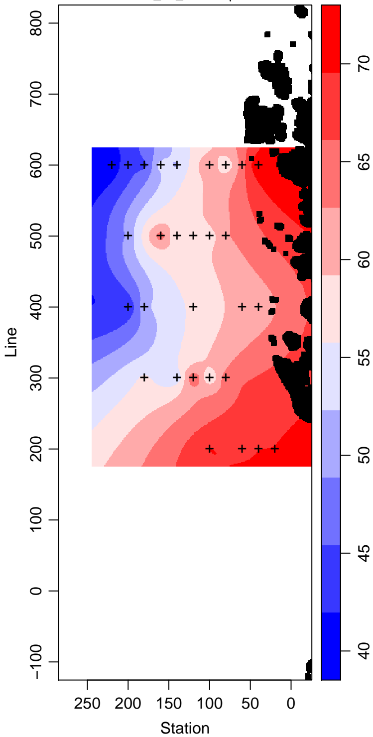
LMG02-01_45_Silicate \mu\text{ mol L}^{-1}
