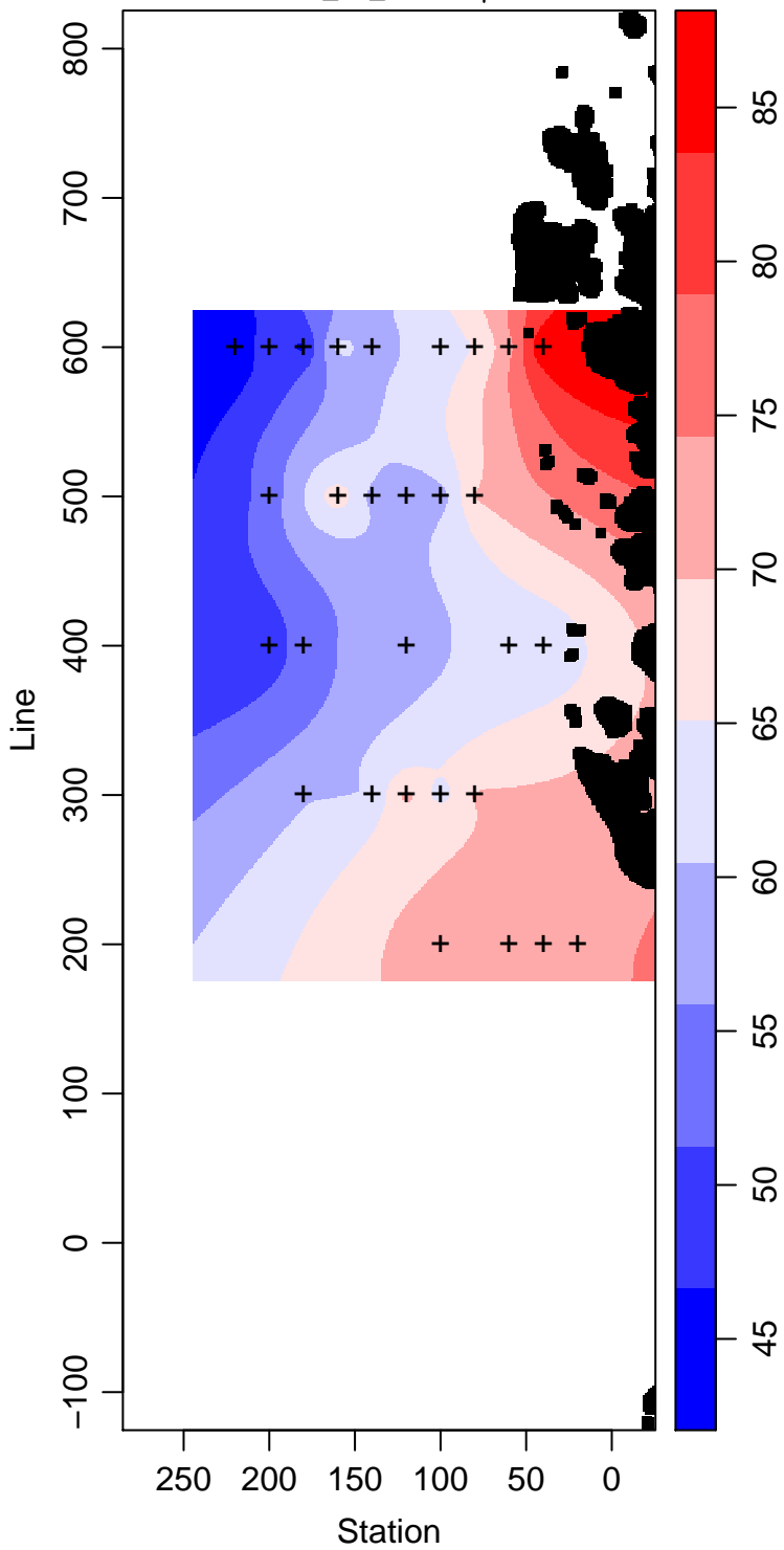
LMG02-01_55_Silicate \mu\text{ mol L}^{-1}
