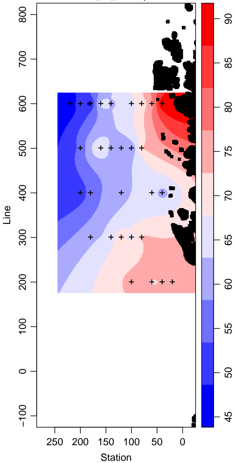
LMG02-01_60_Silicate \mu\text{ mol L}^{-1}
