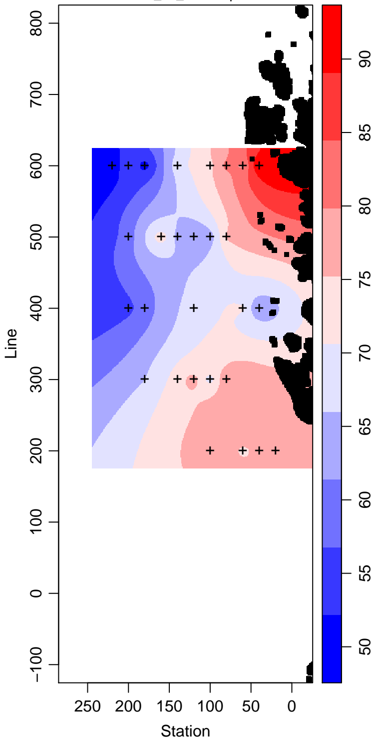
LMG02-01_70_Silicate \mu\text{ mol L}^{-1}
