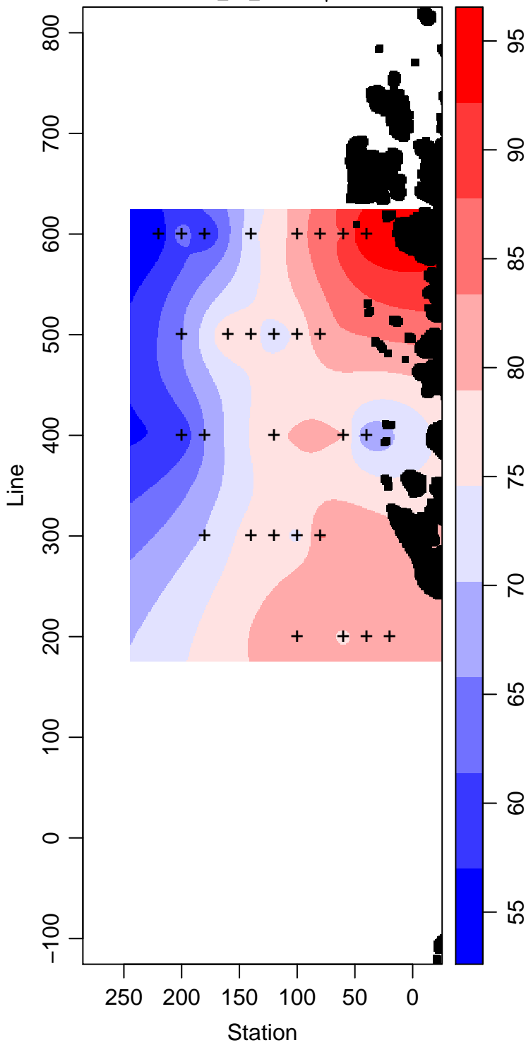
LMG02-01_85_Silicate \mu\text{ mol L}^{-1}
