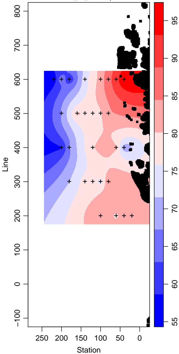
LMG02-01_90_Silicate \mu\text{ mol L}^{-1}
