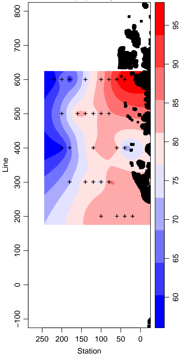
LMG02-01_95_Silicate \mu\text{ mol L}^{-1}
