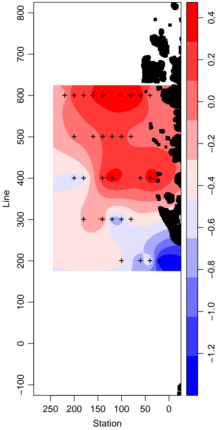
LMG02-01_55_Temperature ° Celsius
