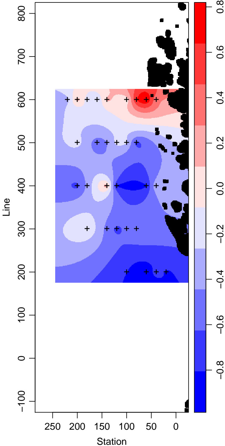
LMG02-01_85_Temperature ° Celsius
