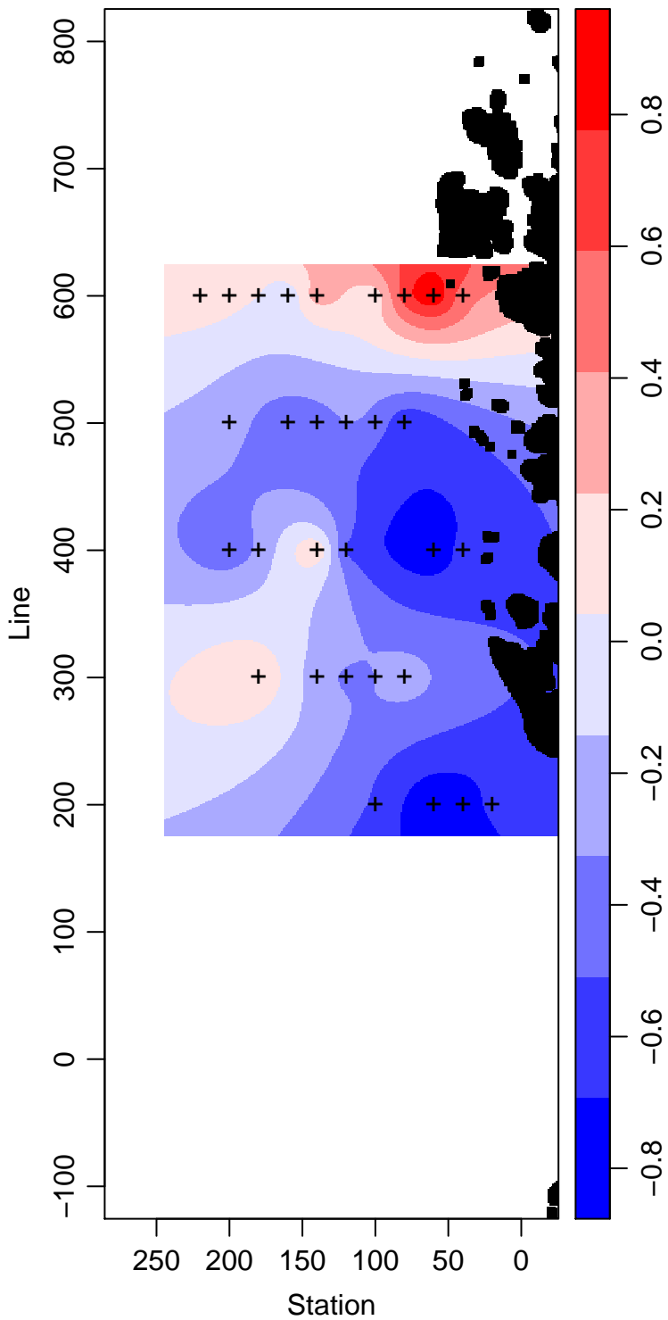
LMG02-01_95_Temperature ° Celsius
