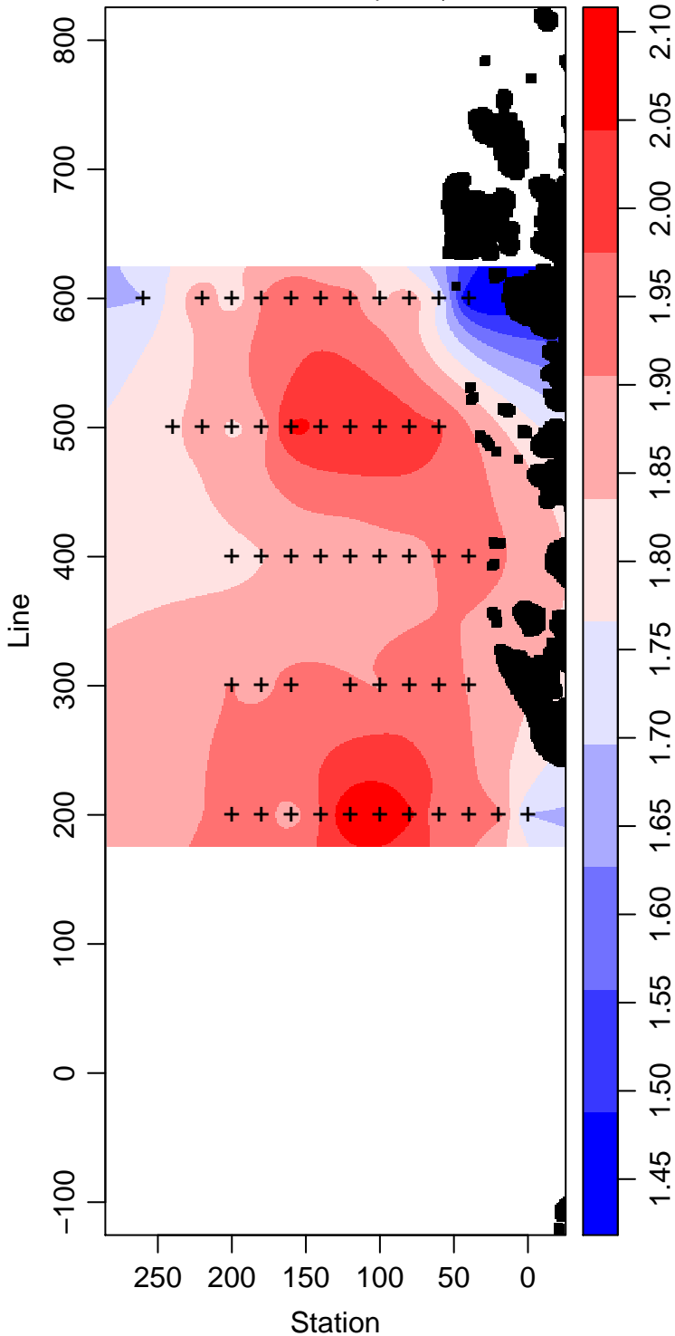
LMG03-01_100_Phosphate \mu\text{ mol L}^{-1}
