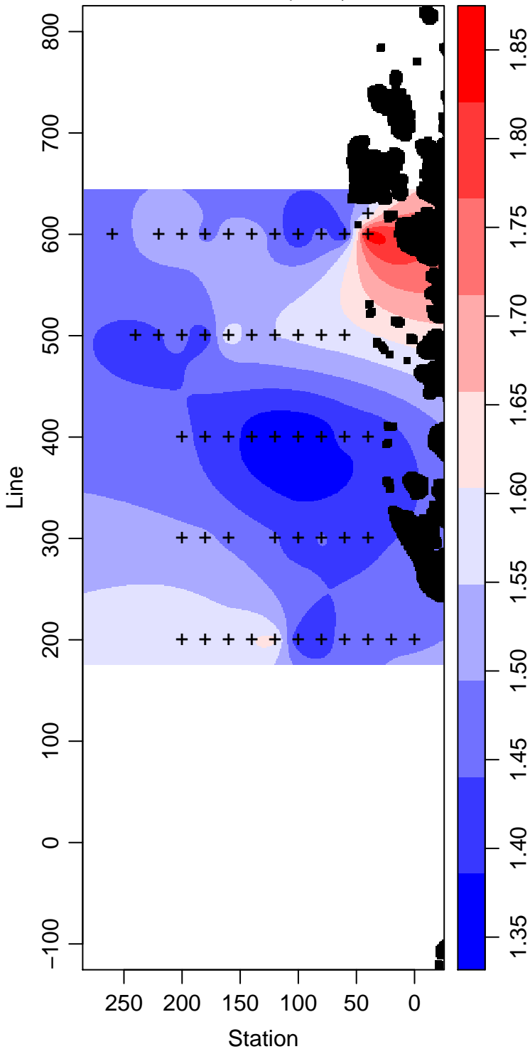
LMG03-01_15_Phosphate \mu\text{ mol L}^{-1}
