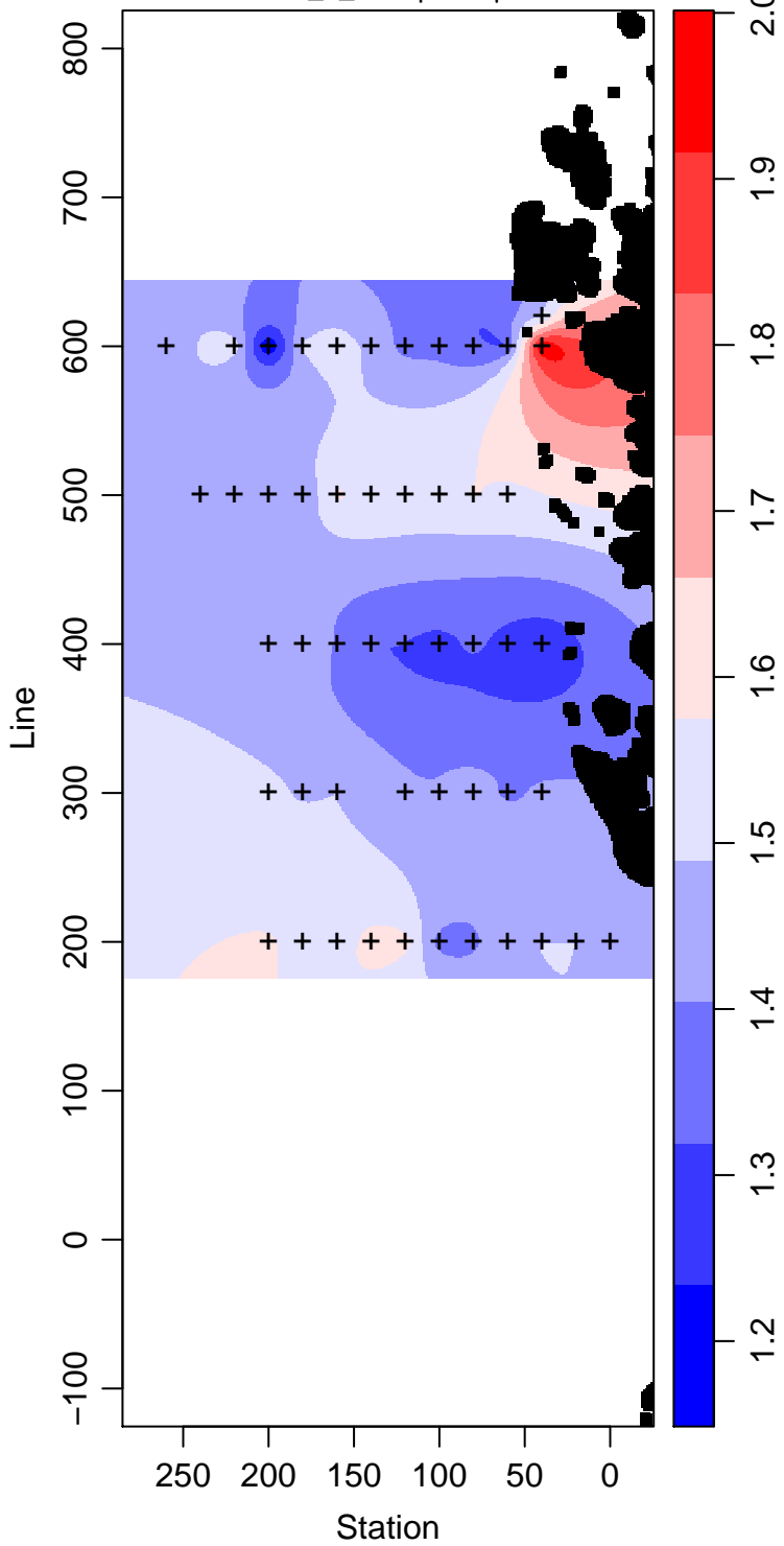
LMG03-01_1_Phosphate \mu\text{ mol L}^{-1}
