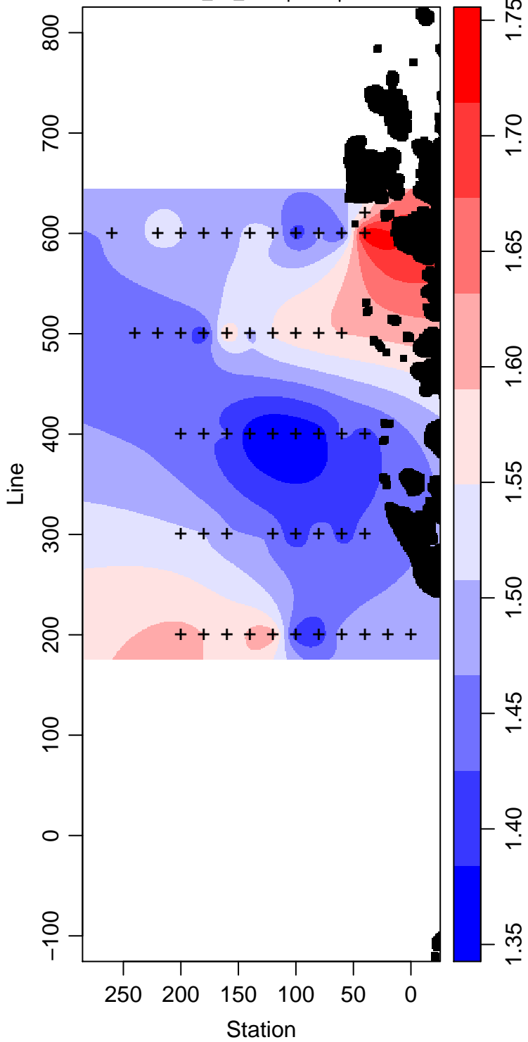
LMG03-01_20_Phosphate \mu\text{ mol L}^{-1}
