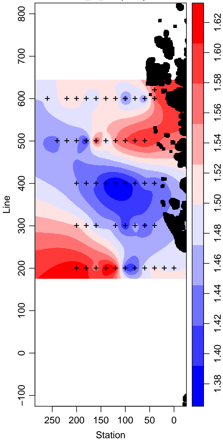
LMG03-01_25_Phosphate \mu\text{ mol L}^{-1}
