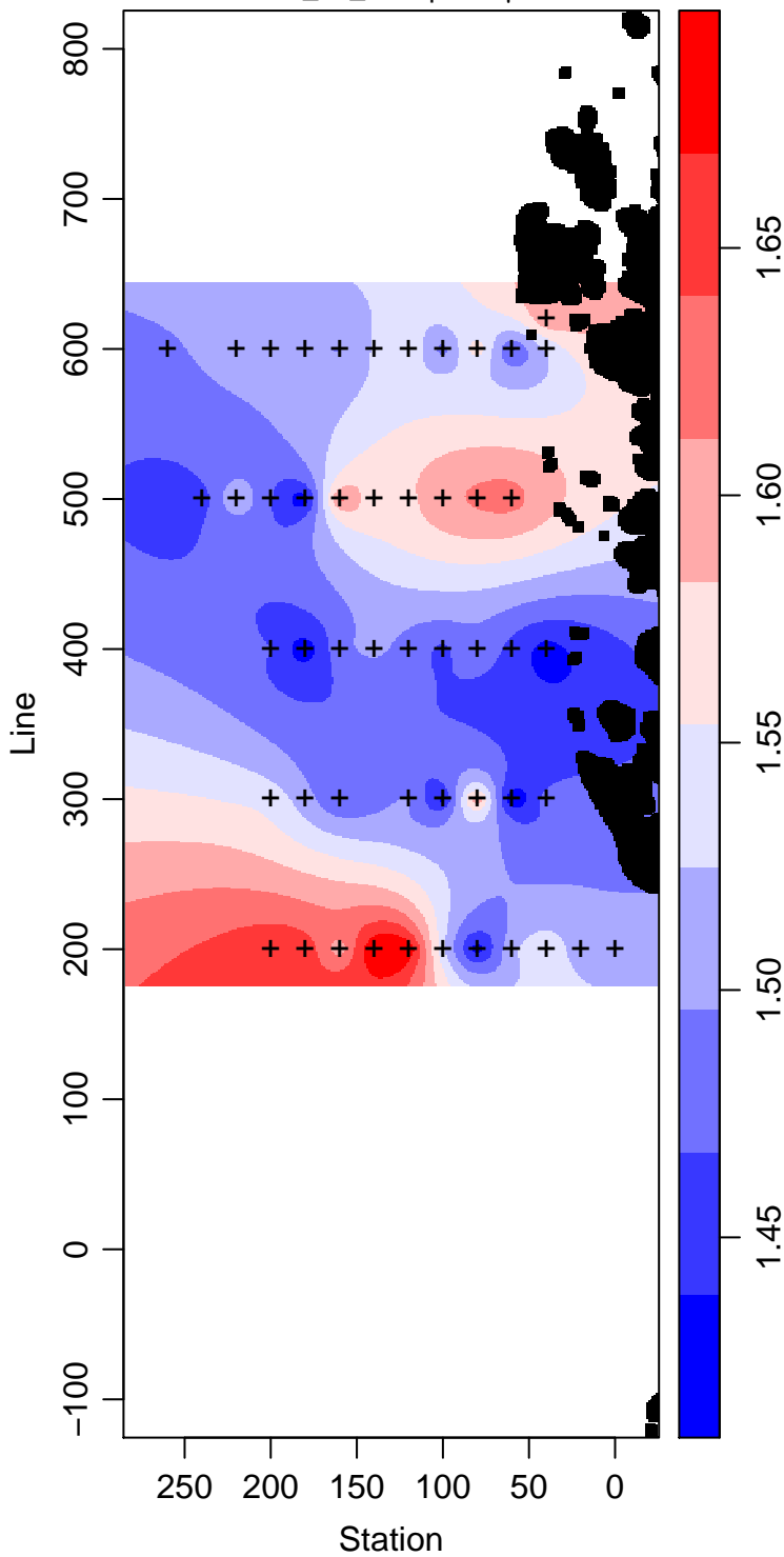
LMG03-01_35_Phosphate \mu\text{ mol L}^{-1}
