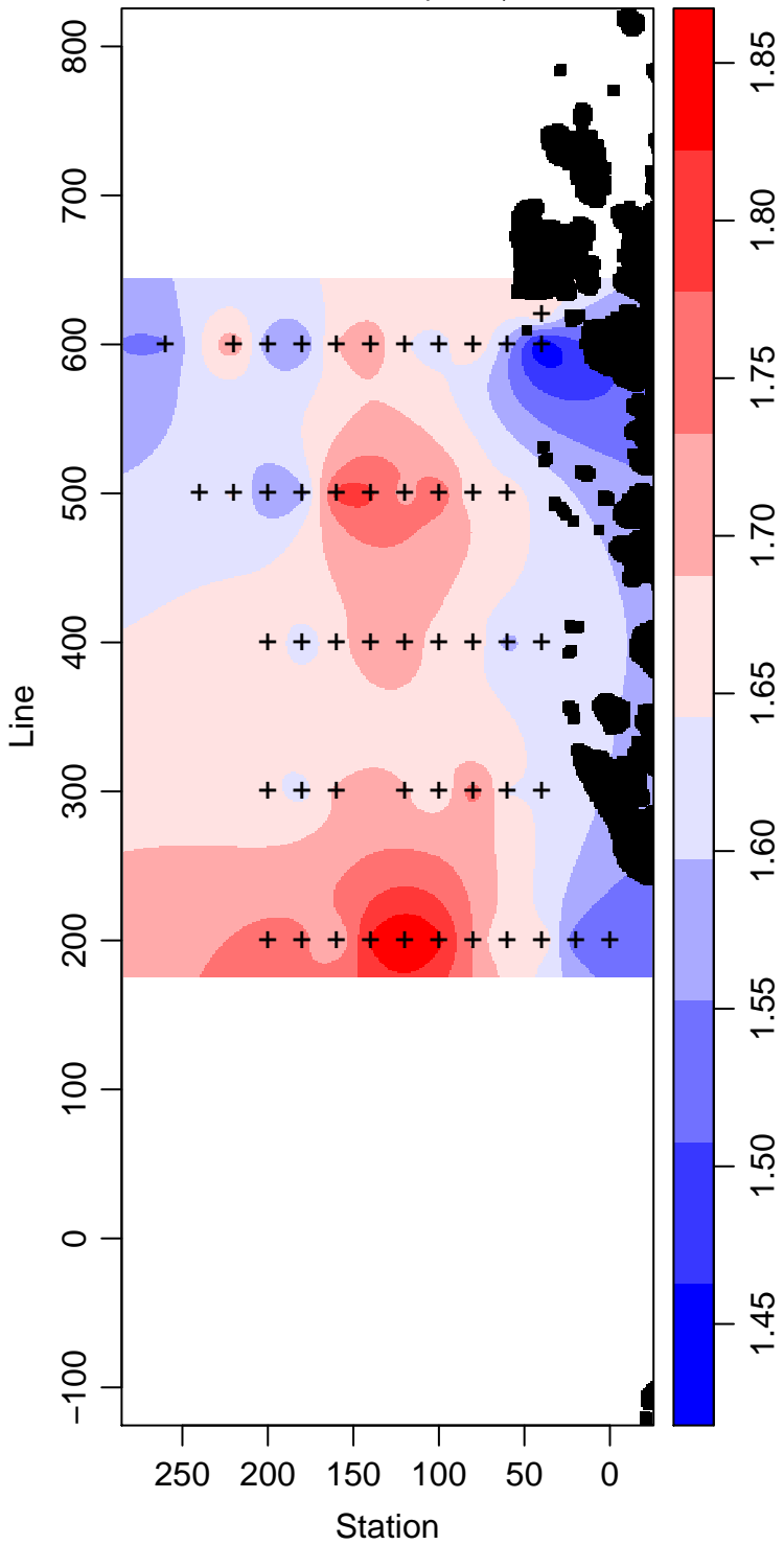
LMG03-01_55_Phosphate \mu\text{ mol L}^{-1}
